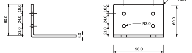
Hang bracket U type
