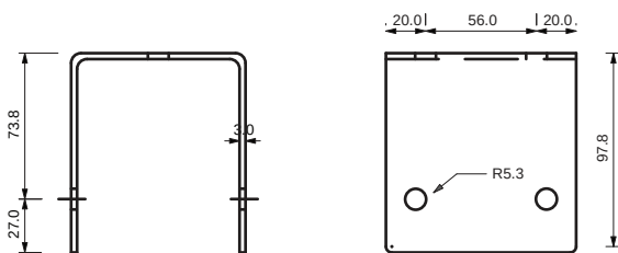
Hang bracket L type
