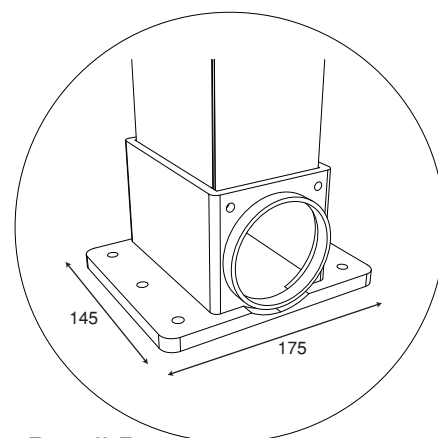
Detail D
